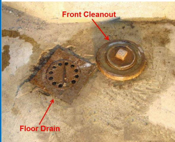
Example of a front sewer cleanout and floor drain
