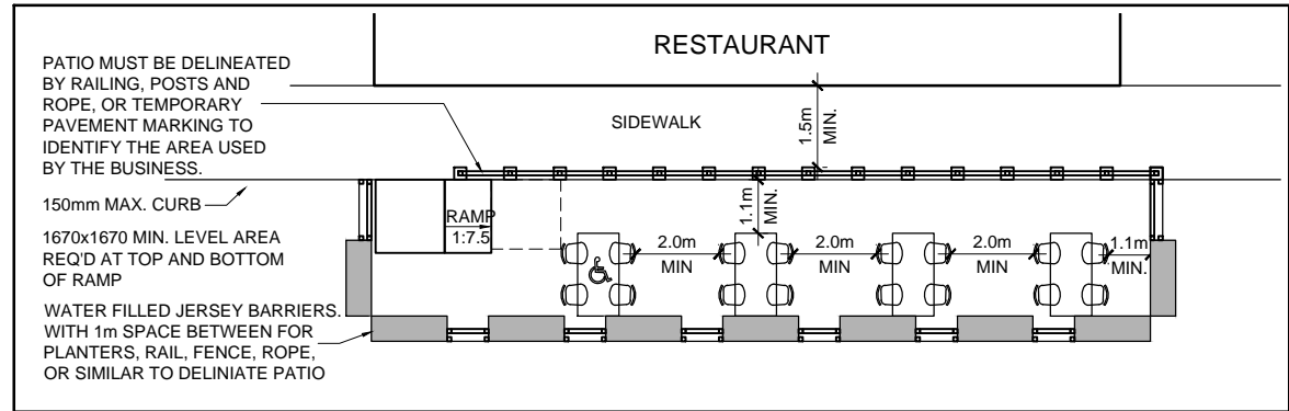
PATIO ON ASPHALT LANE - EXAMPLE 3 (For Narrow Sidewalks)
