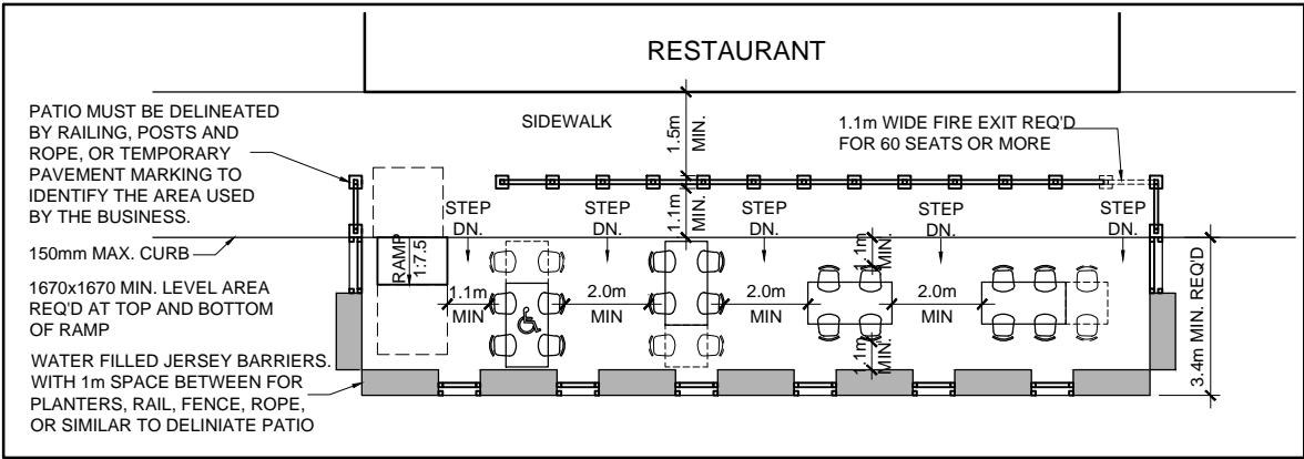
PATIO ON ASPHALT LANE - EXAMPLE 2 (Wide lane width req'd)
