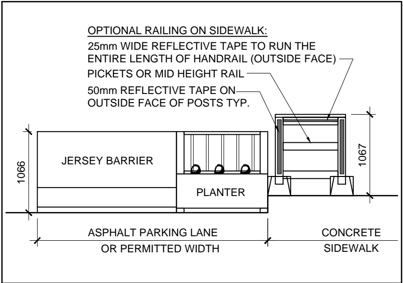
SIDE ELEVATION - EXAMPLE
