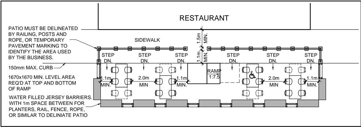
PATIO ON ASPHALT LANE - EXAMPLE 1
