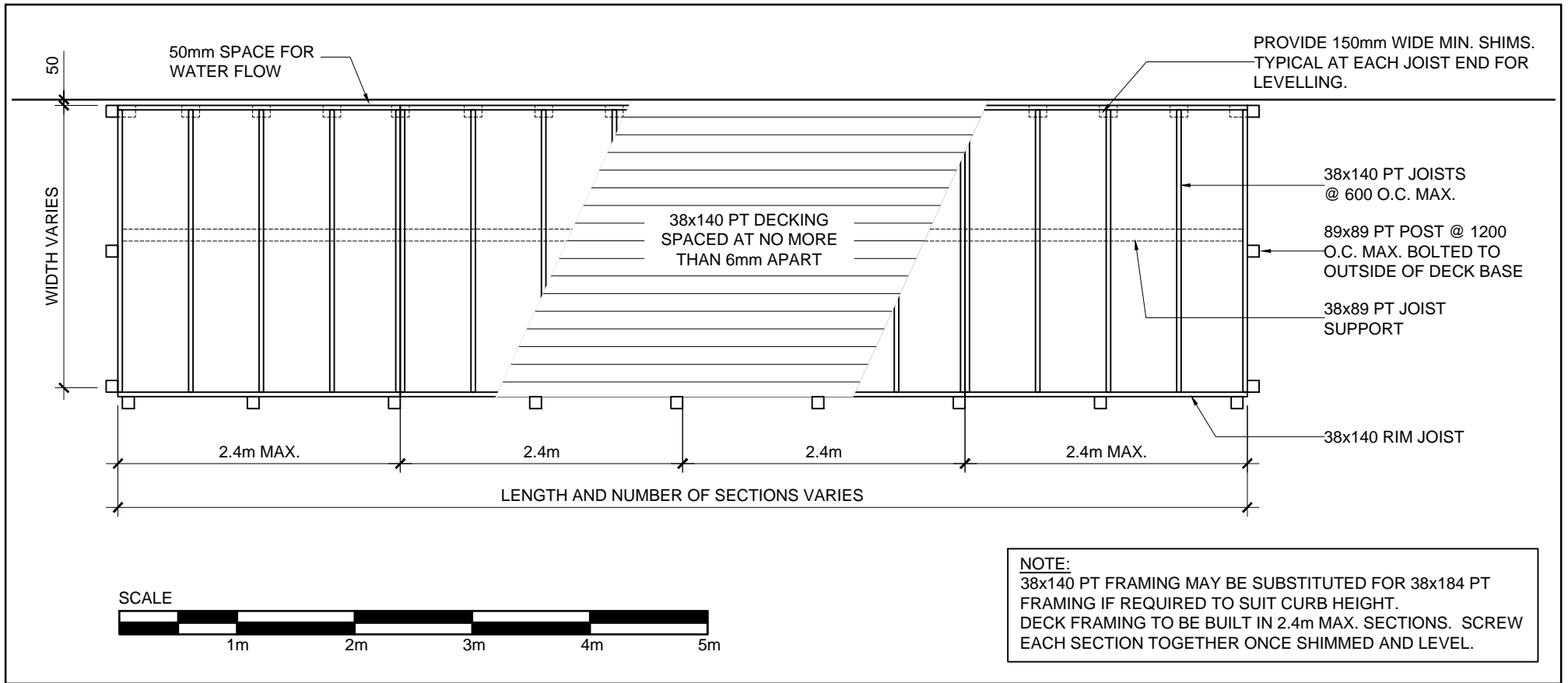
DECK FRAMING PLAN
