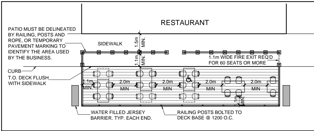
DECK PATIO - EXAMPLE 1
