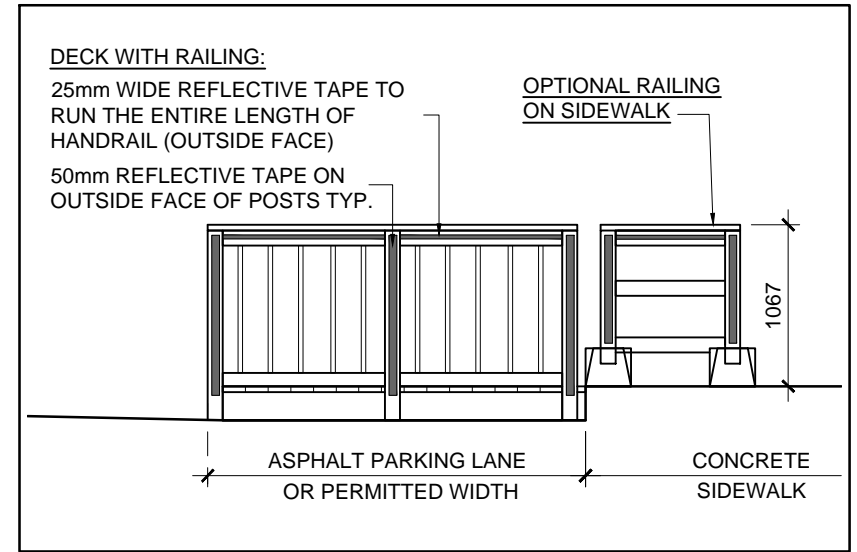
SIDE ELEVATION - EXAMPLE
