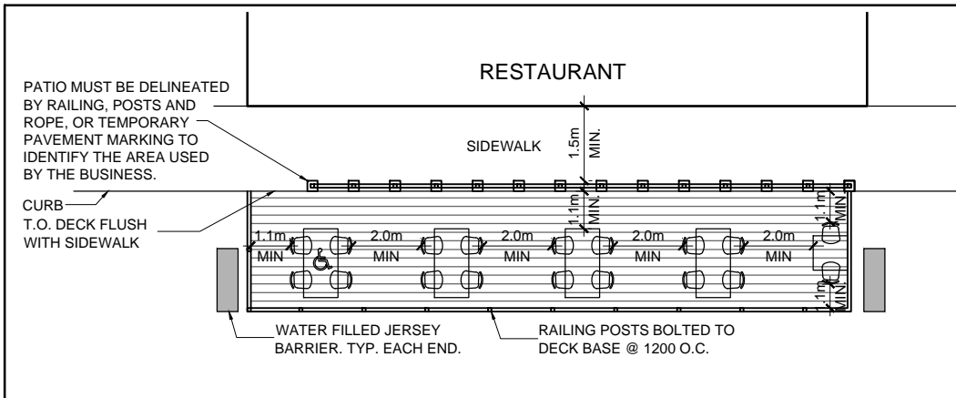
DECK PATIO - EXAMPLE 2 (For Narrow Sidewalks)
